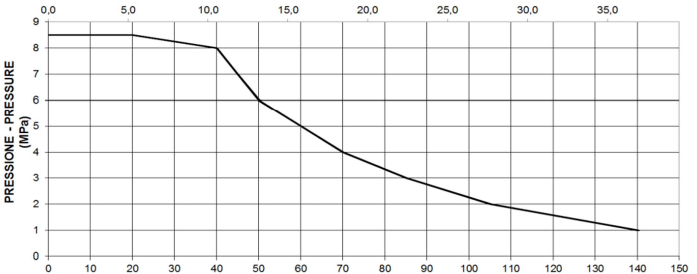
DIAGRAMMA PORTATA - PRESSIONE PRESSURE-FLOW RATE DIAGRAM
